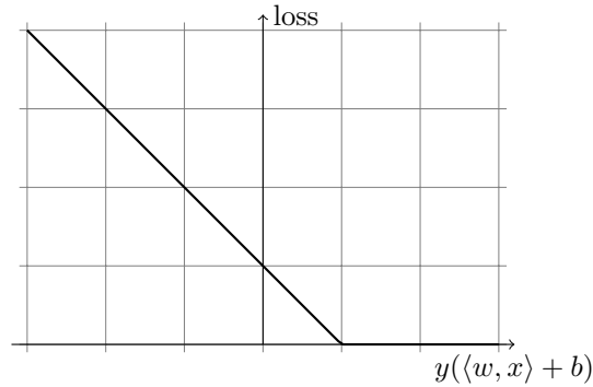
Fig. 7.3. The binary hinge loss. Note that the loss is convex but non-differentiable at the kink point. Furthermore, it increases linearly as the distance from the decision hyperplane y(\langle w, x \rangle + b) decreases.
